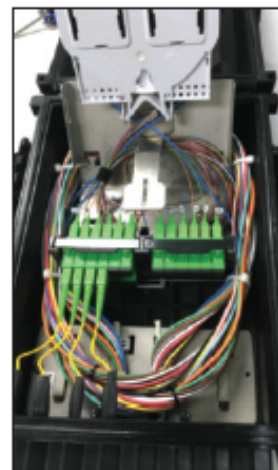
Fiber Loop Storage
